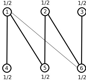
FIGURE 6. Network G_5
