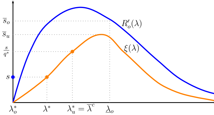
Figure 10: Comparison with large c .
