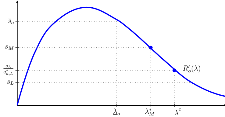
Figure 4: PO scenario with Trade.
